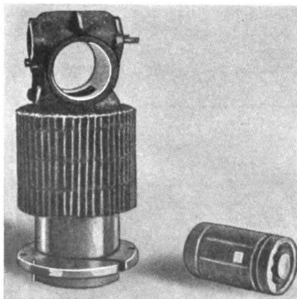
Cylinder and Valve as Actually Made.
